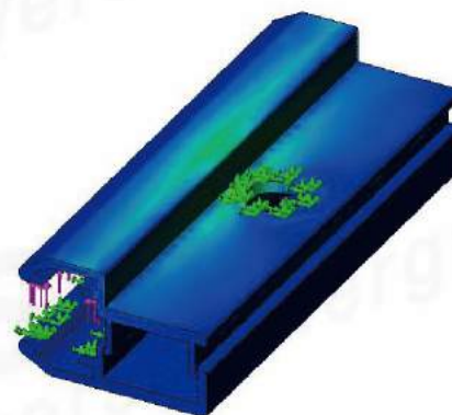
Thin Film End Clamp Stress Nephogram
