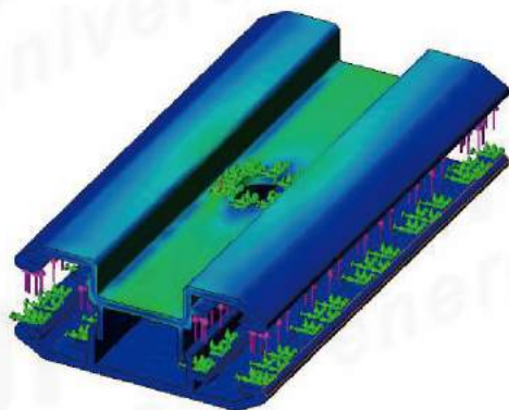
Thin Film Middle Clamp Stress Nephogram
